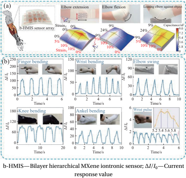
图2 以弹性体材料为基体的MXene传感器用于动作监测： (a) 传感器阵列监测肘部动作示意图；(b) 监测手指、手腕、肘部、膝盖、脚踝、脉搏 [47-48] Fig. 2 MXene sensors based on elastomer materials used for motion monitoring: (a) Schematic diagram of sensor array monitoring elbow movements; (b) Monitoring of fingers, wrists, elbows, knees, ankles and pulse [47-48]
