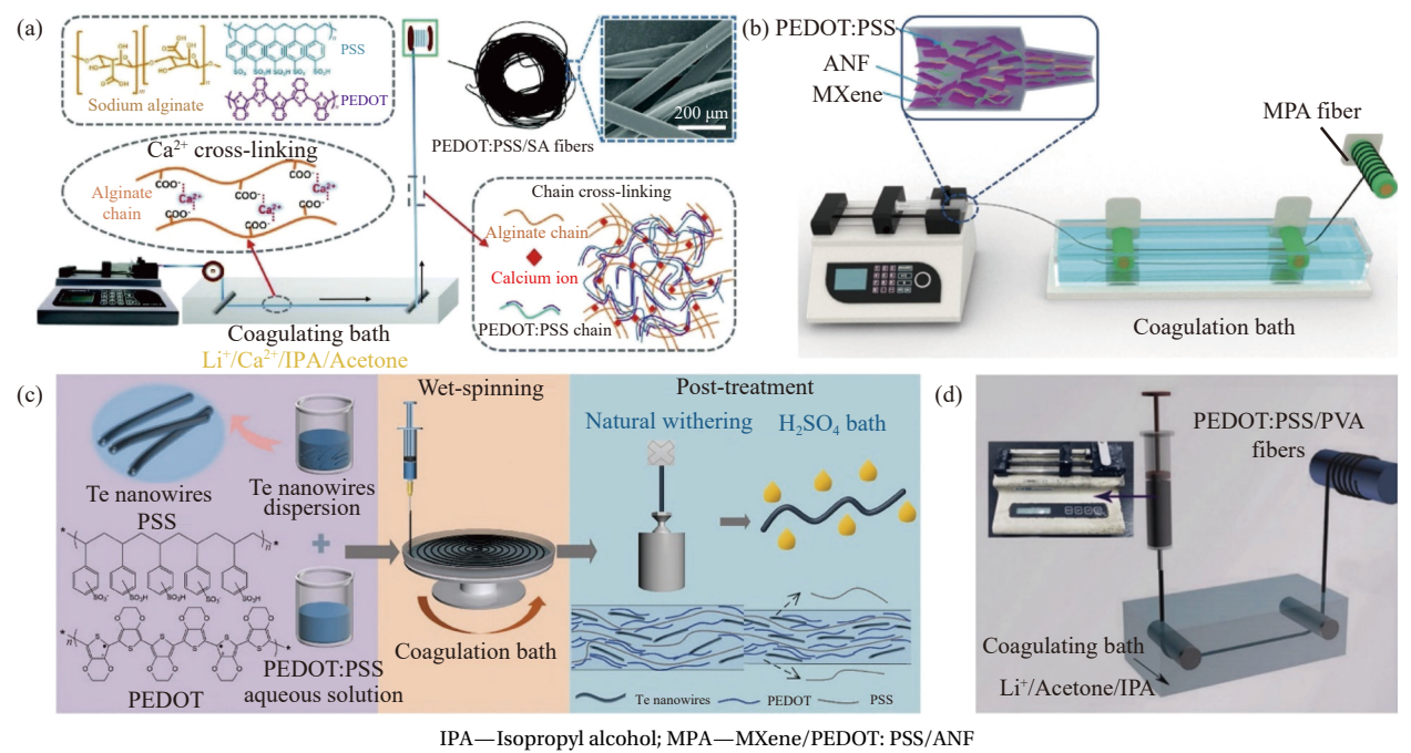
图2 不同组分纺丝液的设计: (a) 海藻酸钠 (SA)/PEDOT:PSS [32] ; (b) 过渡金属碳氮化物 (MXene)/PEDOT:PSS/芳纶纳米纤维 (ANF) [33] ; (c) 碲纳米线 (TeNWs)/PEDOT:PSS [34] ; (d) 聚乙烯醇 (PVA)/乙二醇 (EG)/PEDOT:PSS [31] Fig. 2 Design of spinning solutions with different components: (a) Sodium alginate (SA)/PEDOT:PSS [32] ; (b) Transition metal carbonitride (MXene)/PEDOT:PSS/Aramid nanofibers (ANF) [33] ; (c) Te nanowires (TeNWs)/PEDOT:PSS [34] ; (d) Polyvinyl alcohol (PVA)/Ethylene glycol (EG)/PEDOT:PSS [31]
