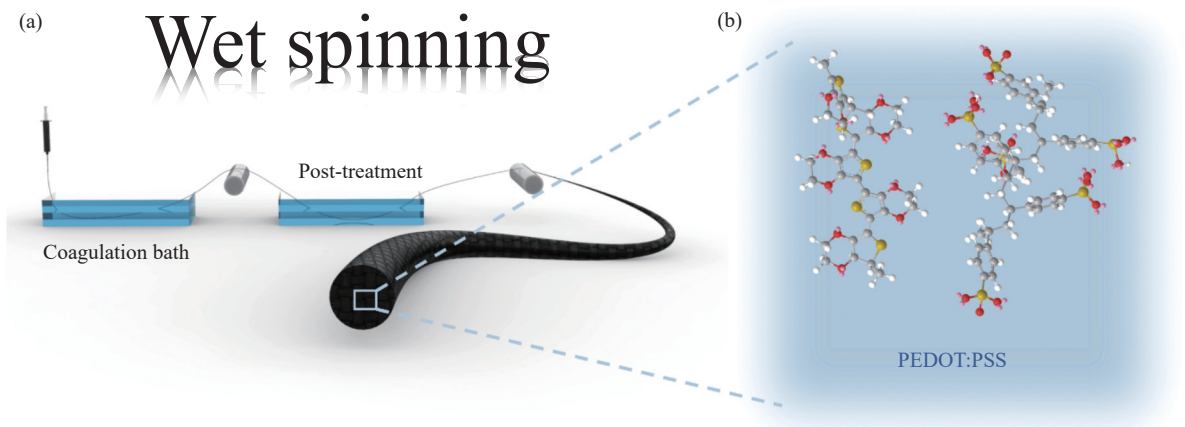
图 1 (a) 湿法纺丝连续制备聚(3, 4-乙烯二氧噻吩):聚(苯乙烯磺酸盐)(PEDOT:PSS) 基纤维的工艺示意图; (b) PEDOT:PSS 分子结构式 Fig. 1 (a) Technical diagram for the continuous preparation of poly(3, 4-ethylenedioxythiophene):poly(styrenesulfonate) (PEDOT:PSS)-based fibers by wet spinning; (b) Molecular structure of PEDOT:PSS
